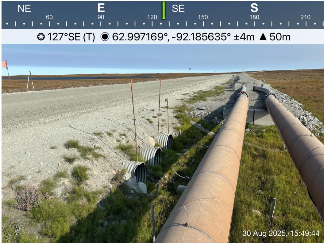
AWAR Road/ Culvert - Photo 69: KM 26.6 Culvert : Outlet.
