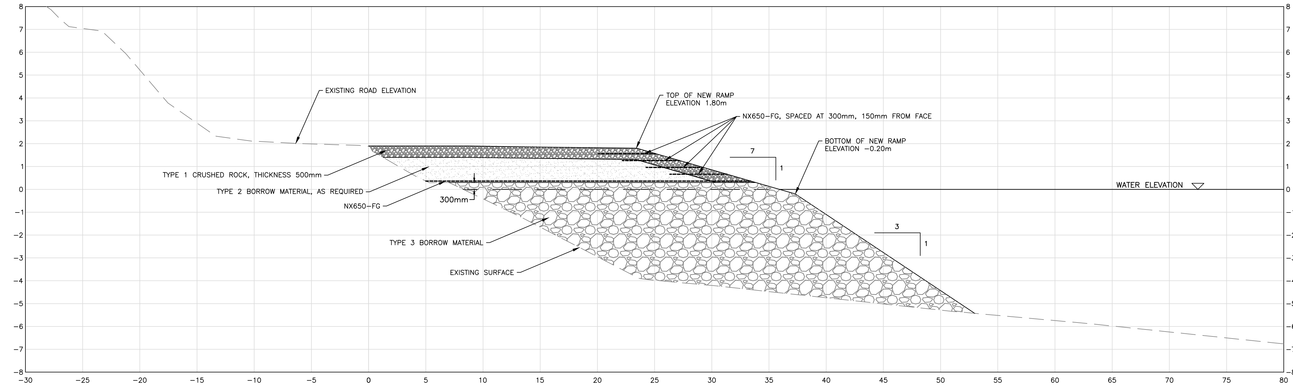
CROSS SECTION 'B' SCALE = 1:1000 HORIZONTAL, 1:500 VERTICAL
